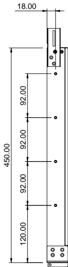
Left-side View
